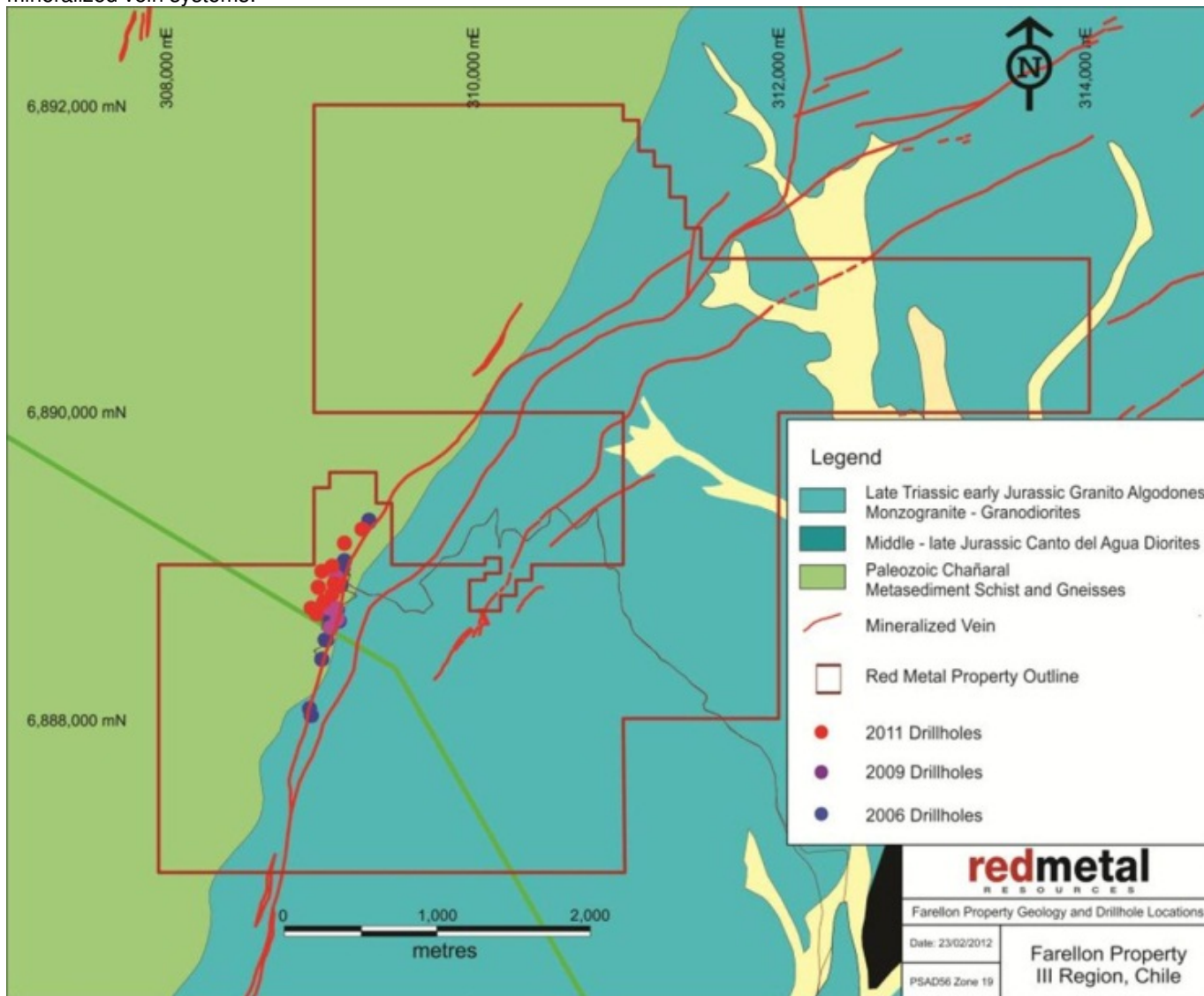
Figure 2: Farellon property geology
